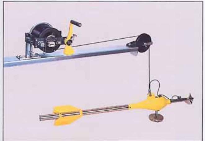
Fig. 6: Cable-suspended meter with jib, 25 kg single-drum winch, Z 215 counter set and 25 kg middle piece.
